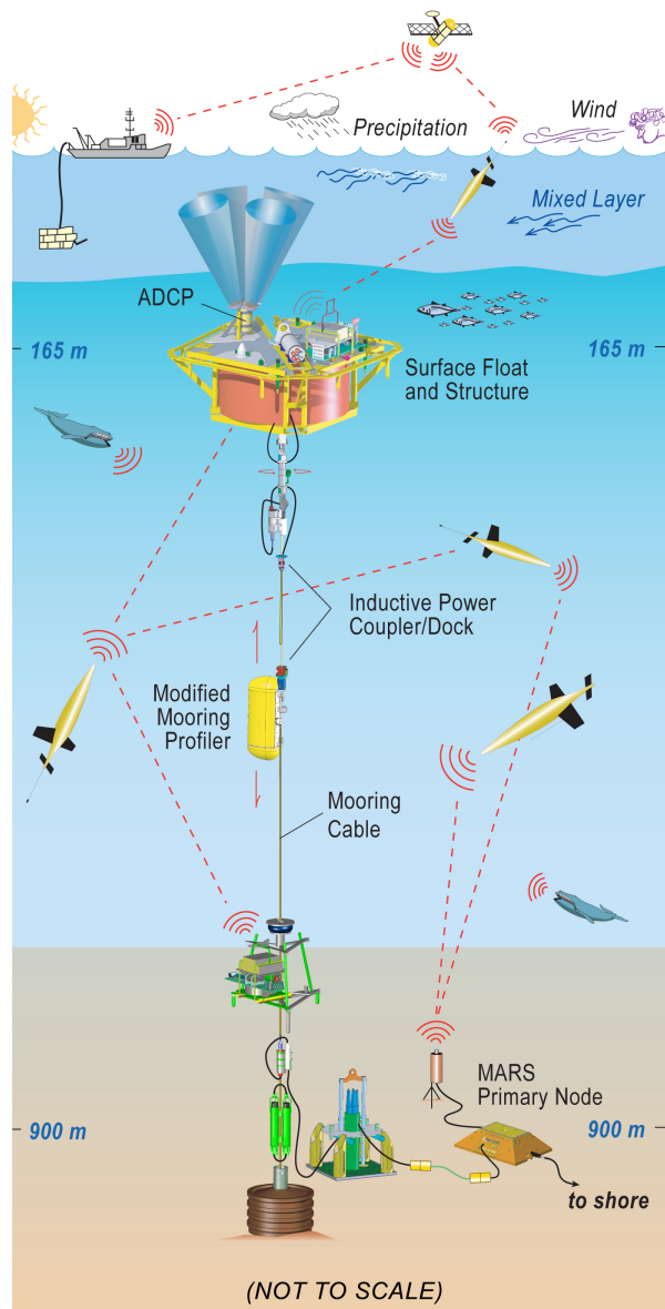
Figure 2: An Ocean observing sensor web system.
