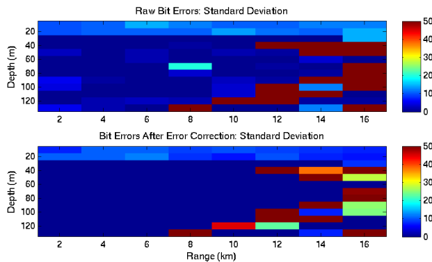
Figure 13: Standard deviations of bit error results over 30 realizations.
