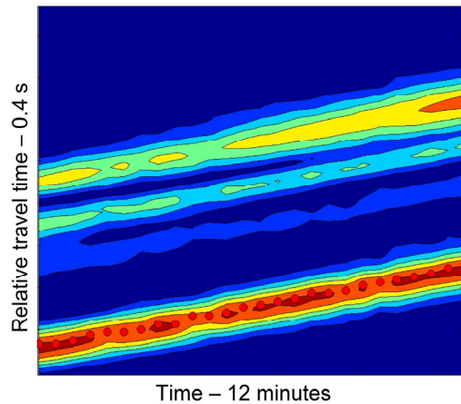
Figure 9: ATOC/NPAL acoustic transmissions received on the acoustic Seaglider.
