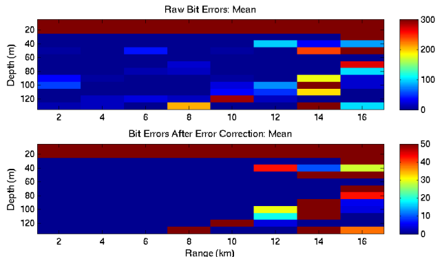
Figure 12: Mean values of bit error results over 30 realizations.
