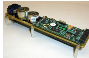
Figure 7: The WHOI MicroModem
