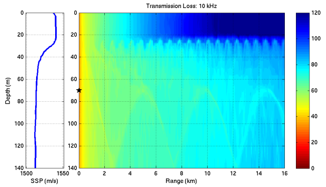
Figure 10: Transmission loss (dB) at 10 kHz for a source at 70m depth.
