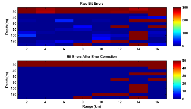
Figure 11: Bit errors as a function of receiver location: raw bit errors in top panel, bit errors after error correction in lower panel. Red in the lower panel indicates failed packet delivery.
